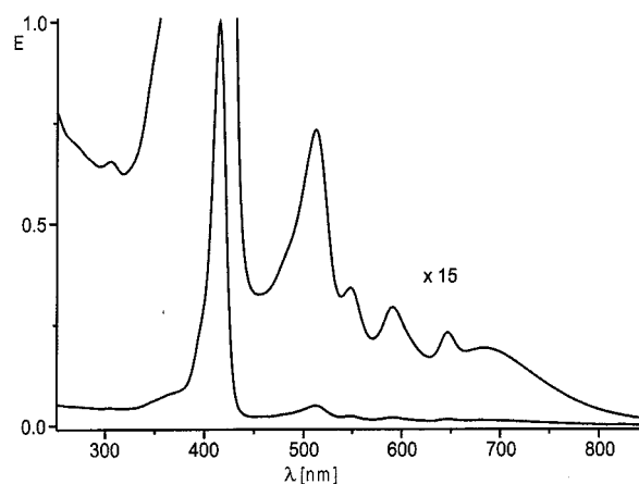
Figure 1. Electronic absorption spectrum of the porphyrin- o -quinone 3 in dichloromethane
