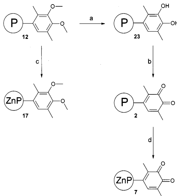
Scheme 4. General reaction scheme for the porphyrin synthesis using the dimethyl compound 12 as an example; a: BBr 3 , CH 2 Cl 2 , -80 °C; b: Ag 2 O; c, d: Zn(ac) 2 , MeOH
