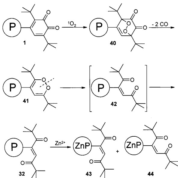
Scheme 9. Putative formation of the porphyrin diketones 32 , 43 and 44
