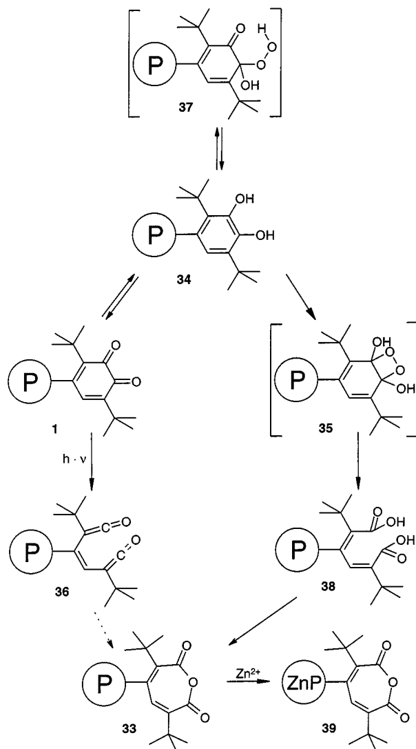
Scheme 8. Possible mechanism for the formation of the muconic acid derivative 33
