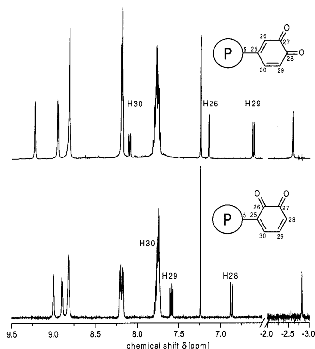
Figure 2. ^1\text{H} -NMR spectra of the two unsubstituted porphyrin- o -quinone isomers 3 and 5
