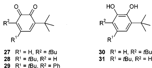
Scheme 6. o -Quinones with high steric demand and their corresponding pyrocatechols
